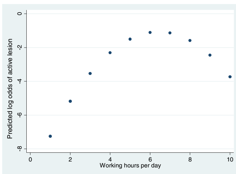
Fig. 1 Relationship between the predicted log odds of an active lesion and hours worked per day. Predicted log odds of active lesion versus number of hours worked per day based on final multilevel multivariable logistic regression model for factors associated with active lesions on elephants from tourism camps in Thailand (all other variables held to referent or mean values)
