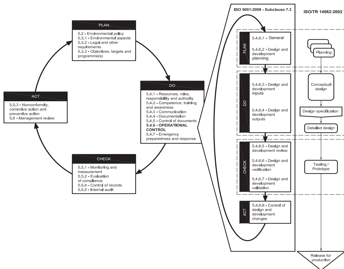
Figure B.1 — Interrelationship between ISO 14006:2011, Clause 5 and other International Standards on ecodesign
