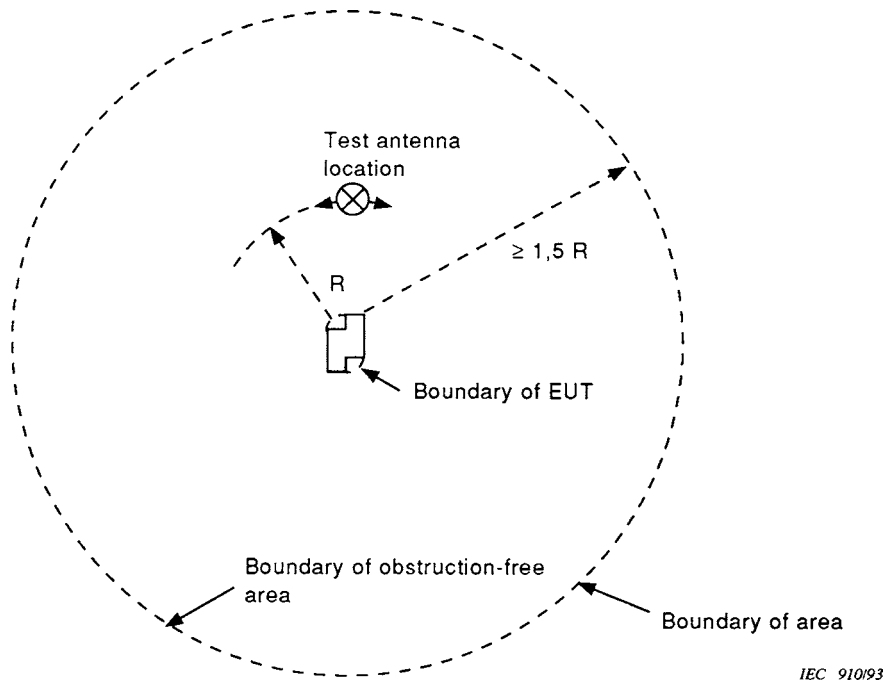
Figure 3 – Obstruction-free area with stationary EUT (see 5.3)
