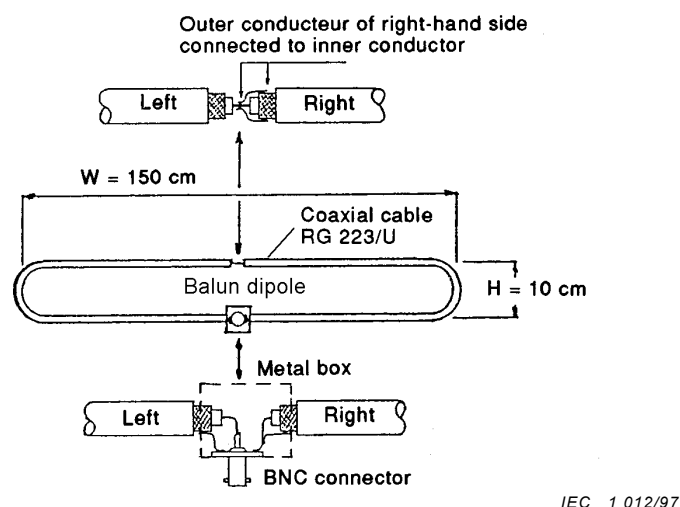
Figure C.9 – Construction of the balun-dipole
