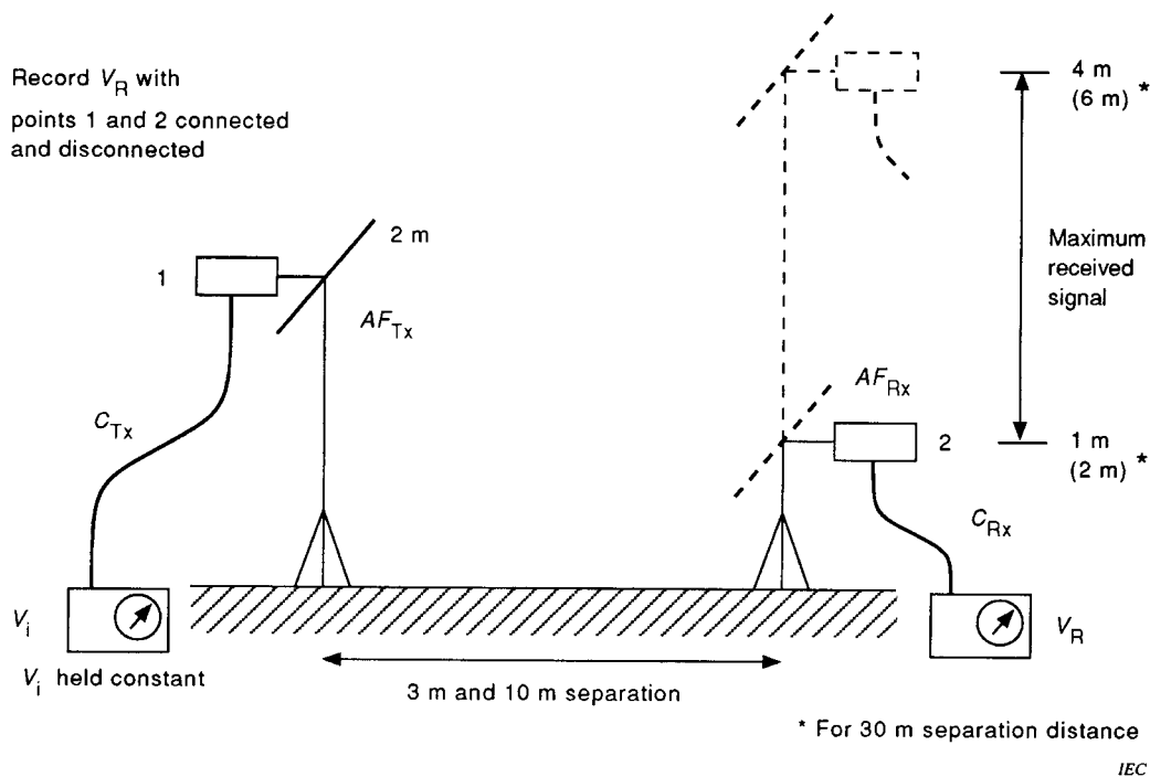
Figure 4 – Configuration of equipment for measuring horizontal polarization of site attenuation (see 5.6 and annex E)
