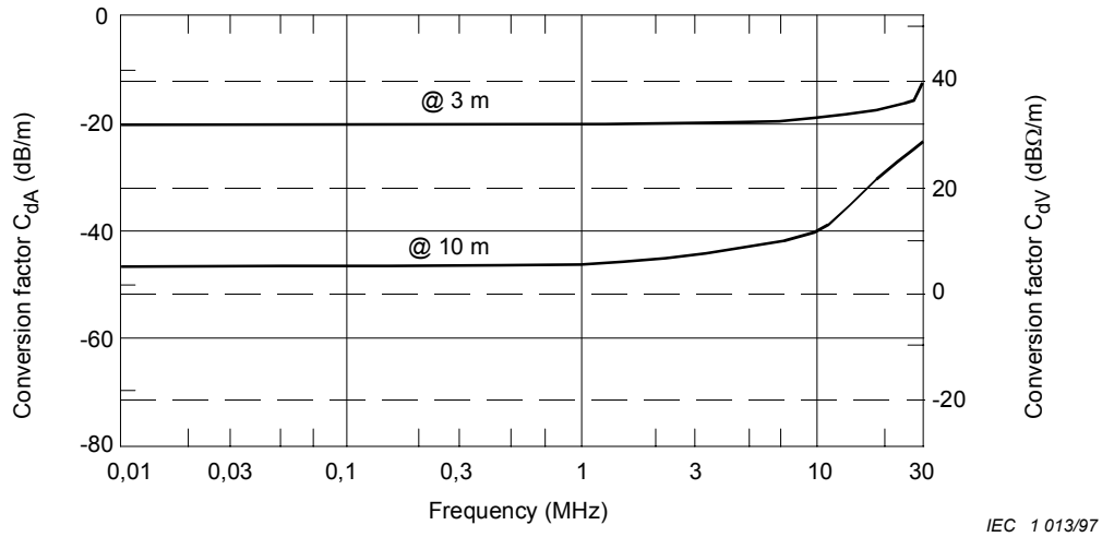
Figure C.10 – Conversion factors C_{dA} (for conversion into dB ( \mu A/m)) and C_{dV} (for conversion into dB ( \mu V/m)) for two standardized measuring distances d
