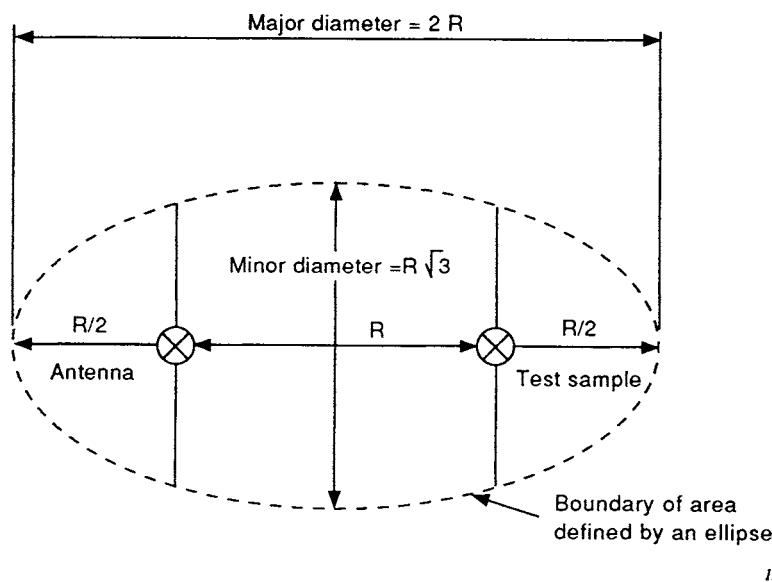
Figure 2 – Obstruction-free area of a test site with a turntable (see 5.3)
