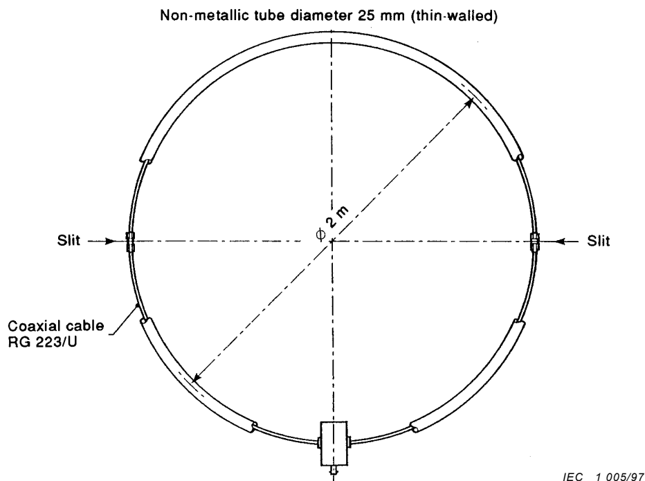
Figure C.2 – A large-loop antenna containing two opposite slits, positioned symmetrically with respect to the current probe C
