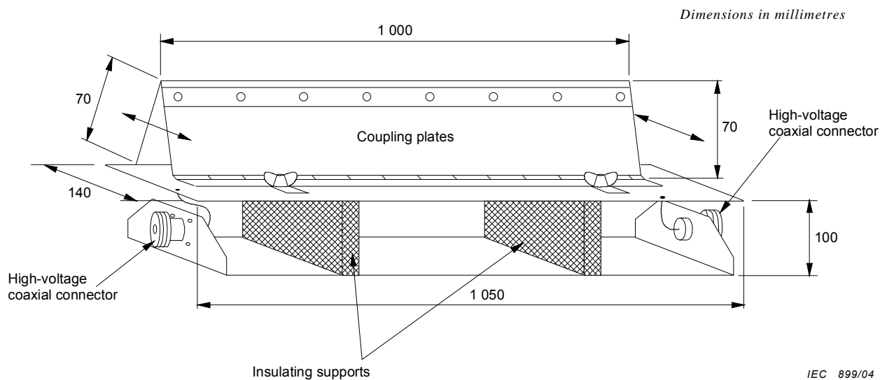
Figure 5 – Construction of the capacitive coupling clamp
