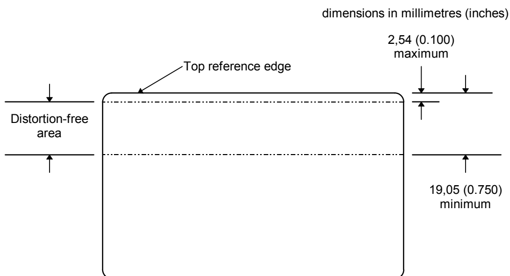
Figure 1 — Distortion-free area on card with magnetic stripe
