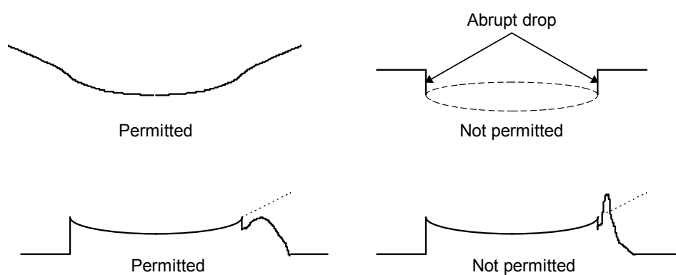
Figure 4 — Surface profile examples
