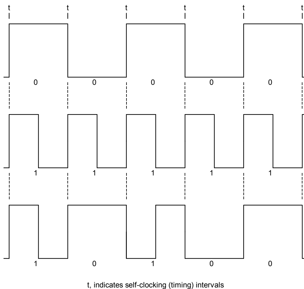
Figure 8 — Examples of two-frequency encoding
