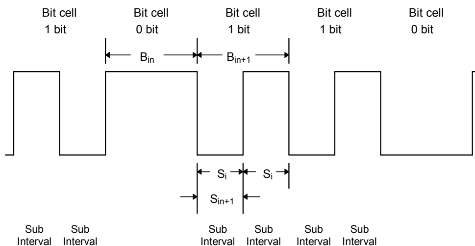
Figure 10 — Flux transition spacing variation
