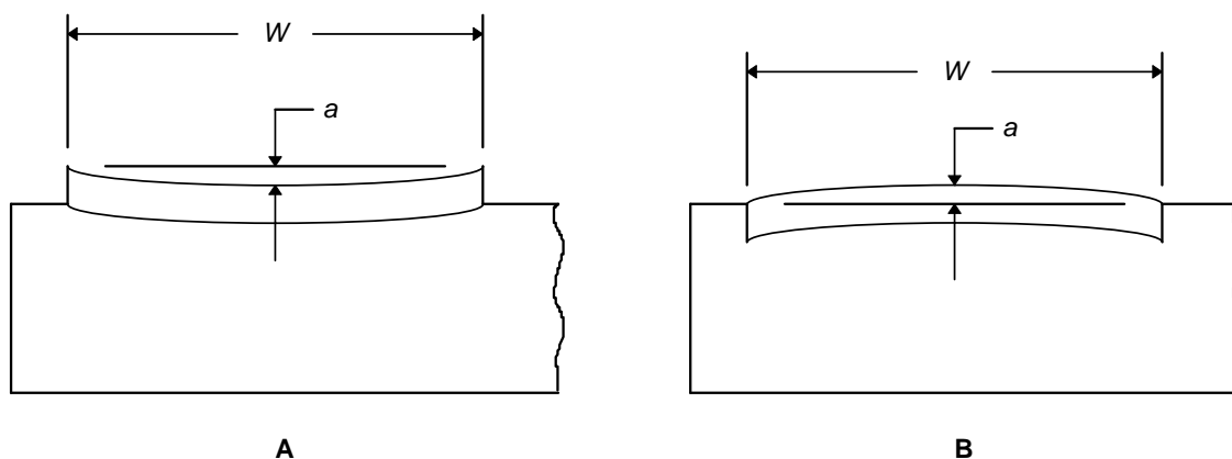
Figure 3 — Surface profile
