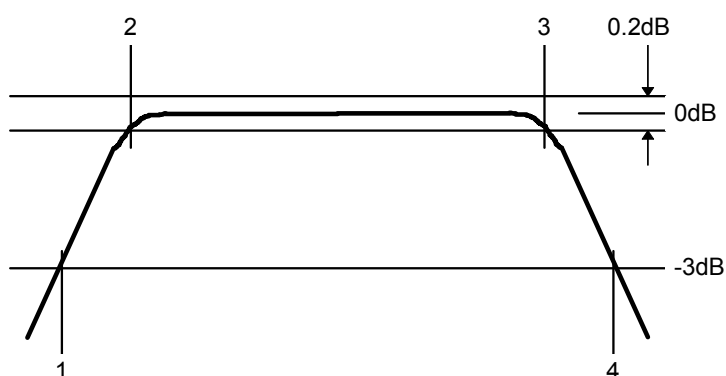
Figure B.1 — Bandpass filter
