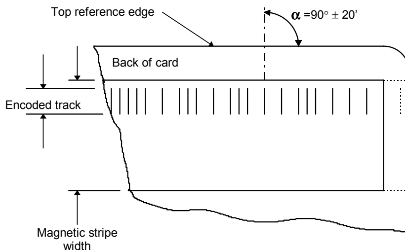
Figure 9 — Angle of recording
