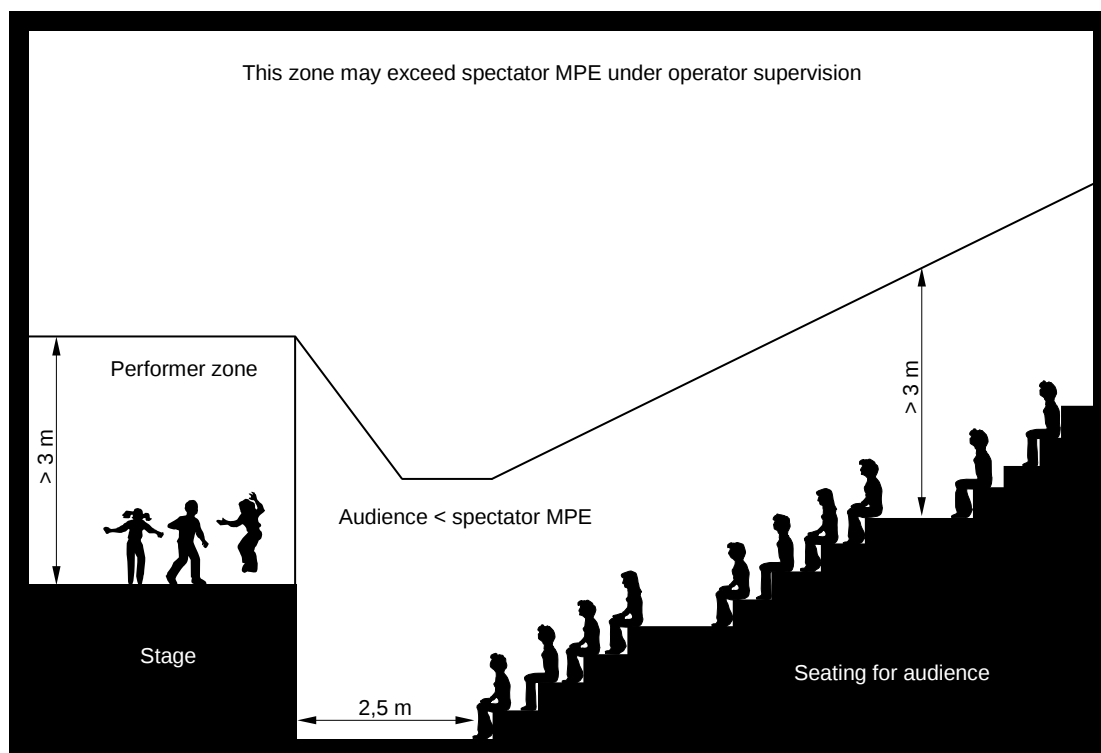
Figure 3 – Audience/spectator separation with operator in control
