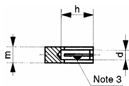
Figure A.7 – Details of socket centre contact
