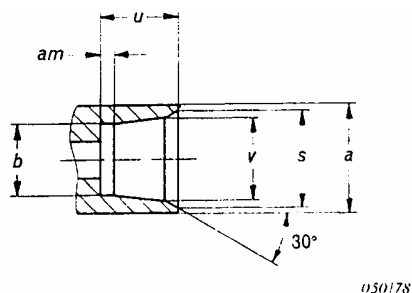
Figure 8 – Gauge for outer contact of pin connector
