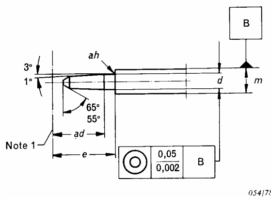
Figure 12 – Dimensions of centre contact (see Table 6)
