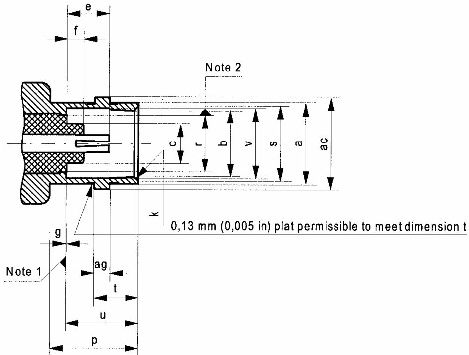
Figure A.5 – Connector with socket centre contact
