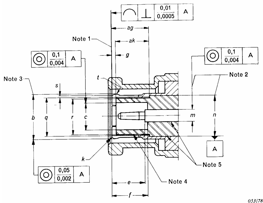
Figure 11 – Dimensions of connector (see Table 6)
