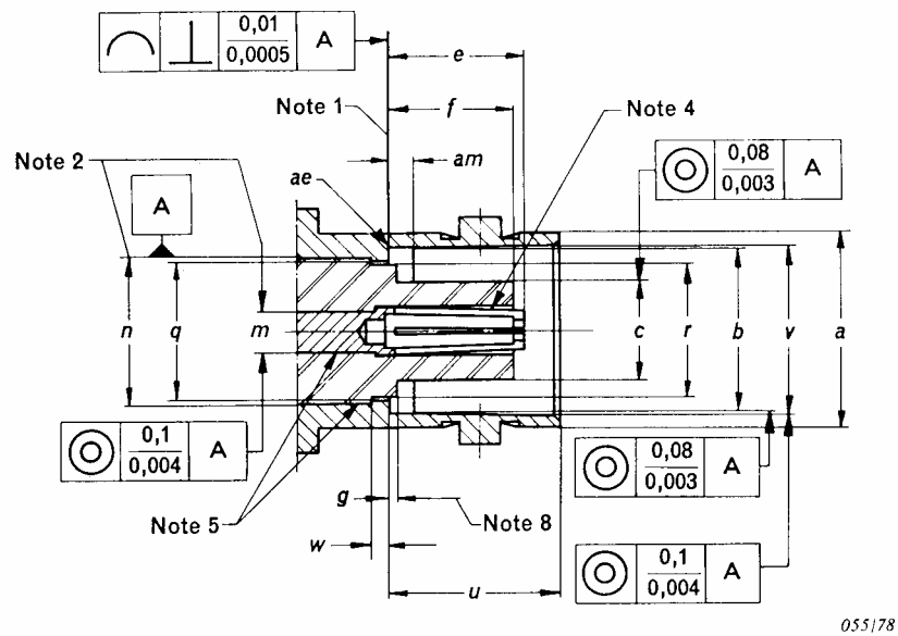
Figure 13 – Dimensions of connector (see Table 7)
