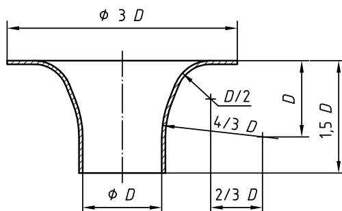
Figure B.10 — Ideal flow orifice
