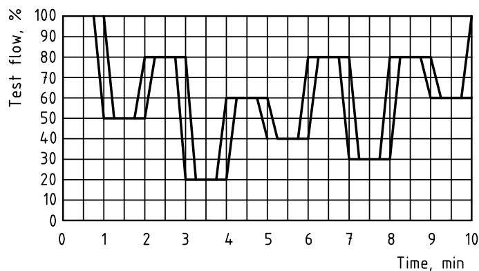
Figure 1 — Typical variable flow cycle (average flow 60 %)
