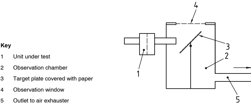
Figure B.17 — Oil carry-over test — Observation chamber
