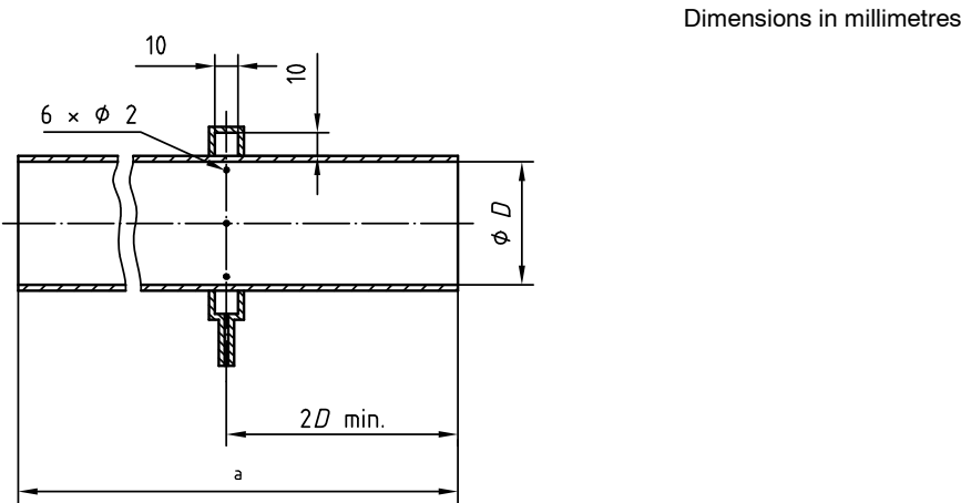
Figure B.3 — ISO heavy-duty dust injector
