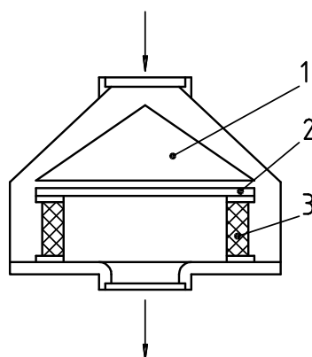
Figure B.5 — Filter element test shroud
