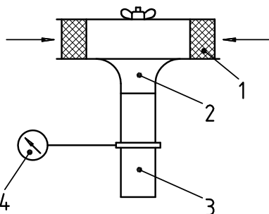
Figure B.9 — Set-up for filter element restriction test
