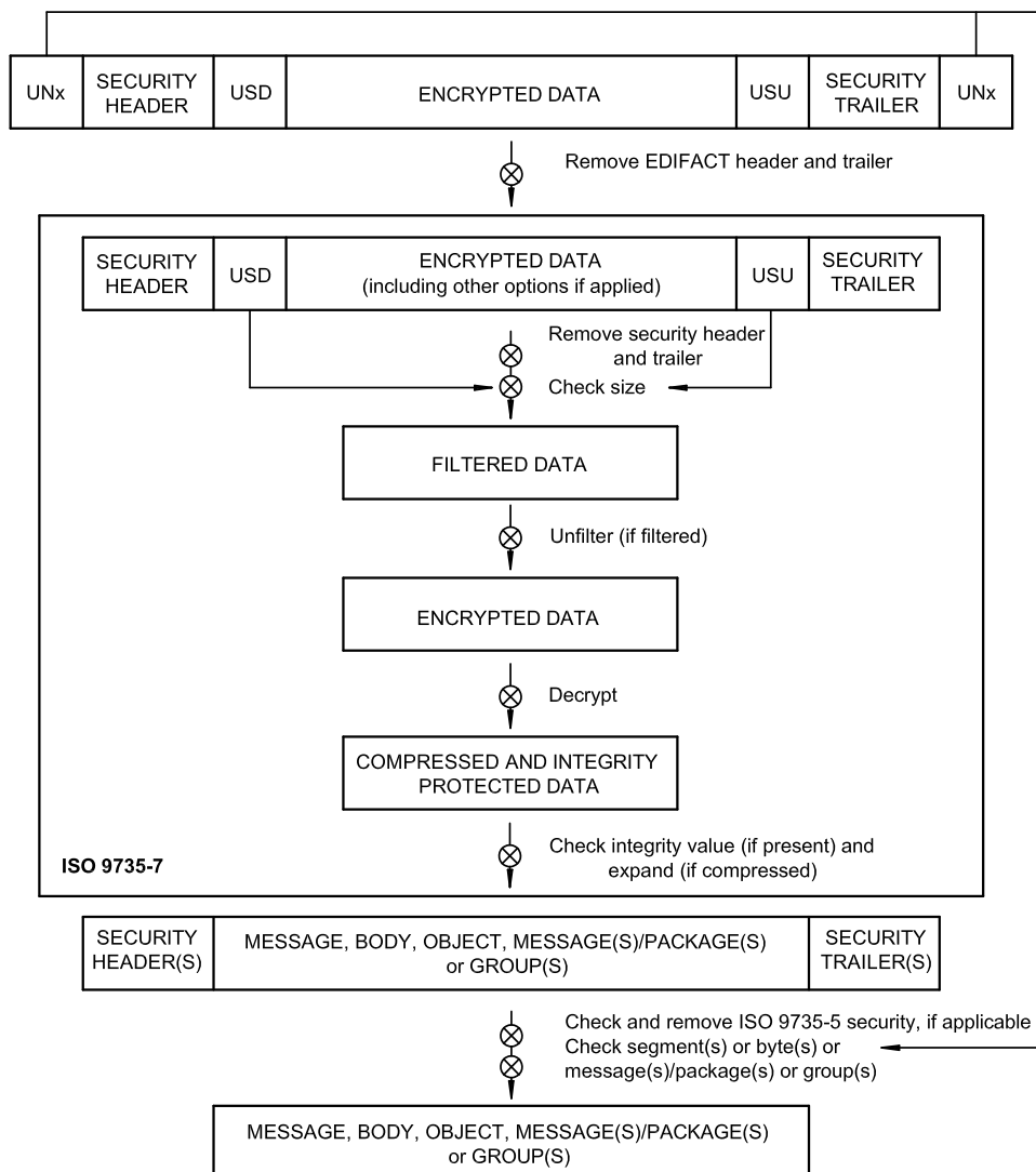
Figure B.2 — Processes involved in decryption of an EDIFACT structure
