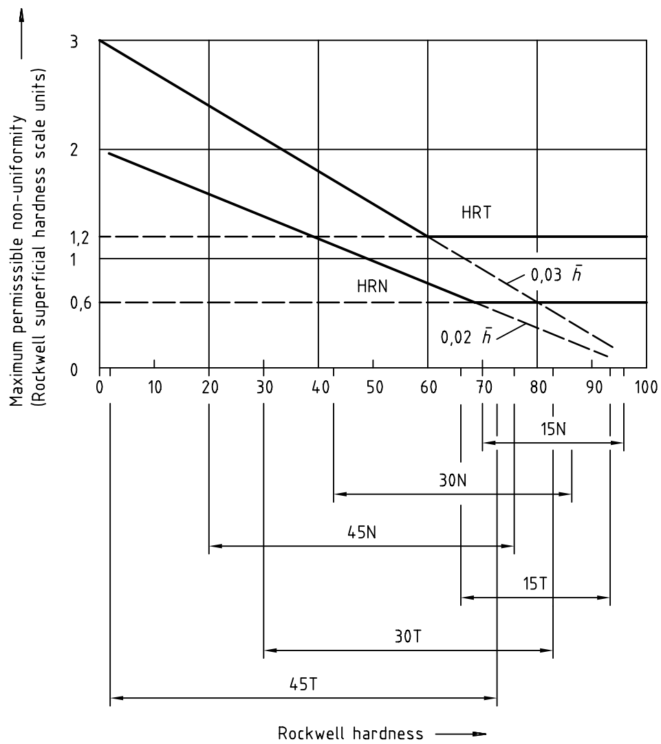
Figure A.2 — Rockwell superficial hardness (scales N and T)
