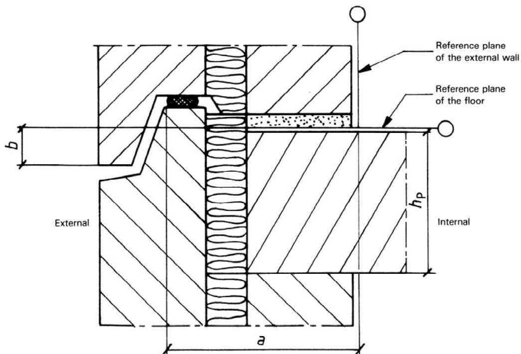
Figure 3 — Cross-section between wall and floor
