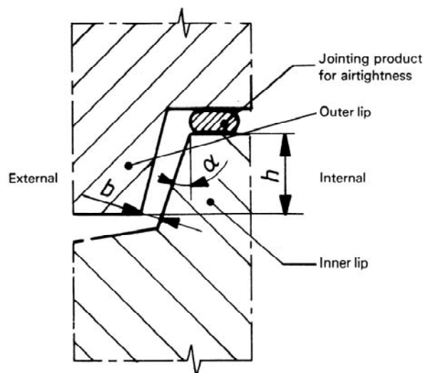
Figure 1 — Cross-section of a horizontal joint
