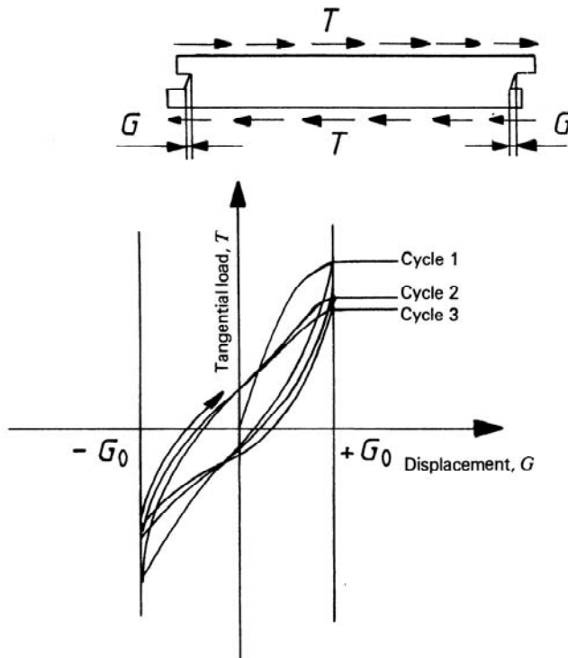
Figure 4 — Example of tangential load-displacement diagram for an alternating shear test with imposed displacement
