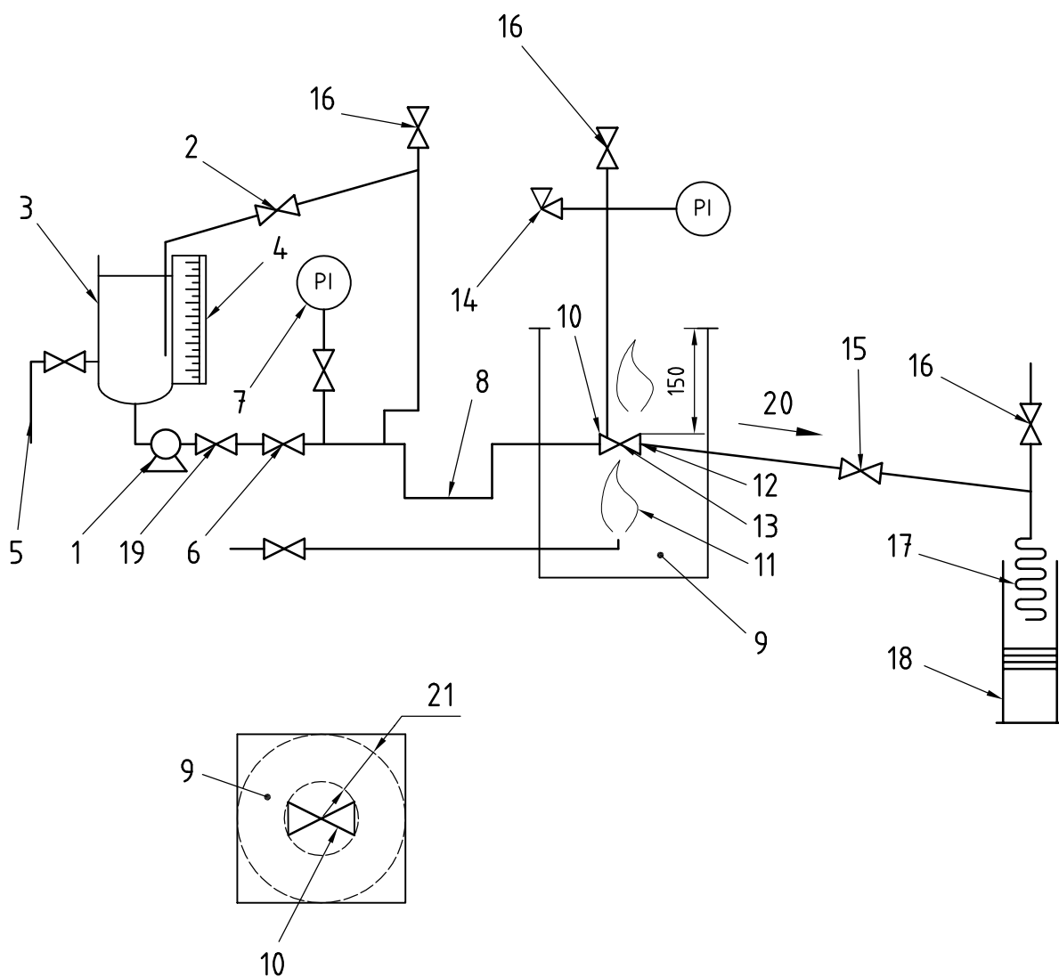
a) Pump as pressure source
