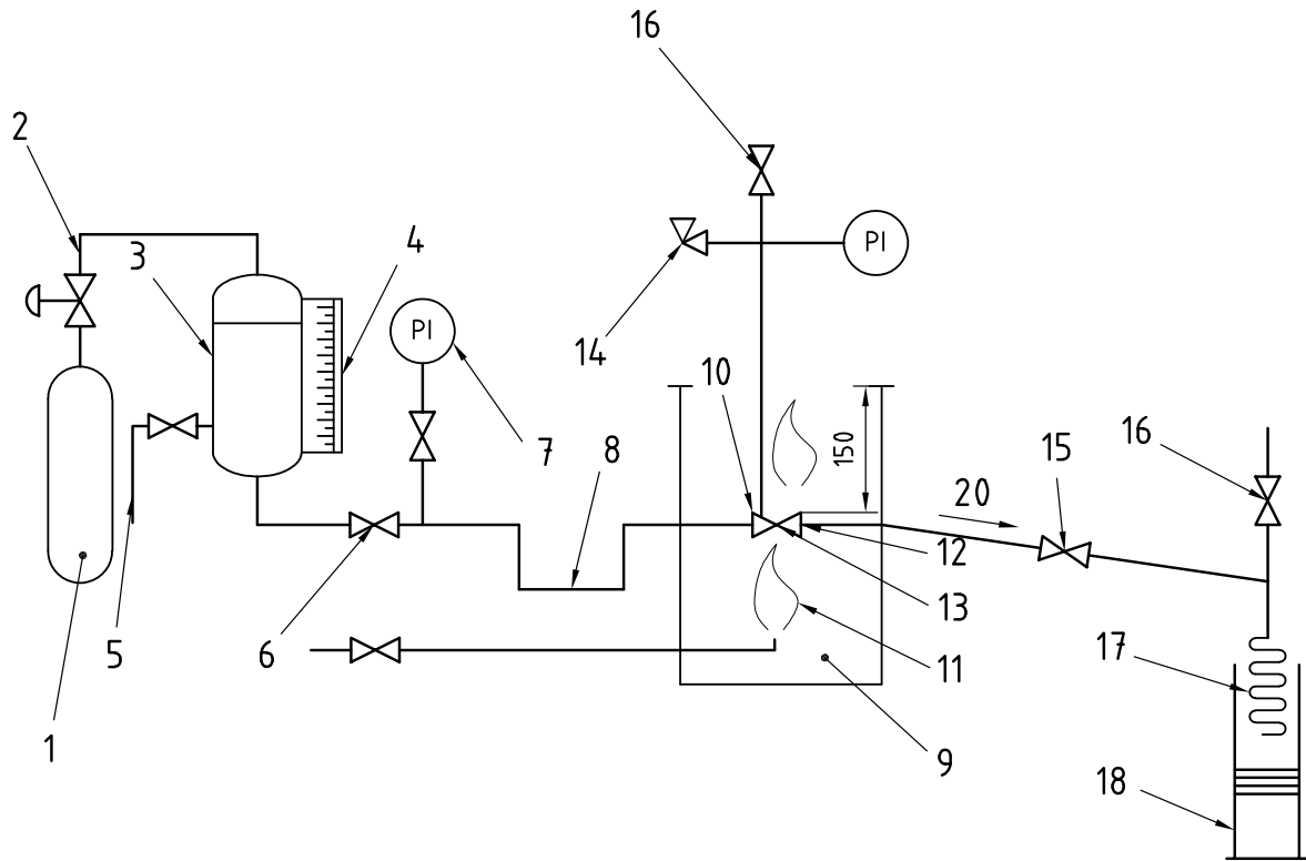
b) Compressed gas as pressure source
