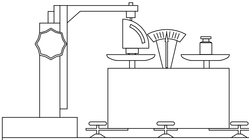
Figure 3 — Apparatus for calibration of durometer spring
