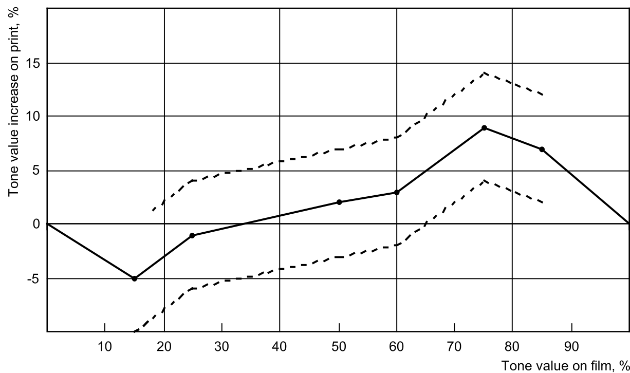
Figure 3 — Typical tone value increase curves for water-based UV and solvent ink (solid) and tolerances (broken), as measured at 30 cm -1
