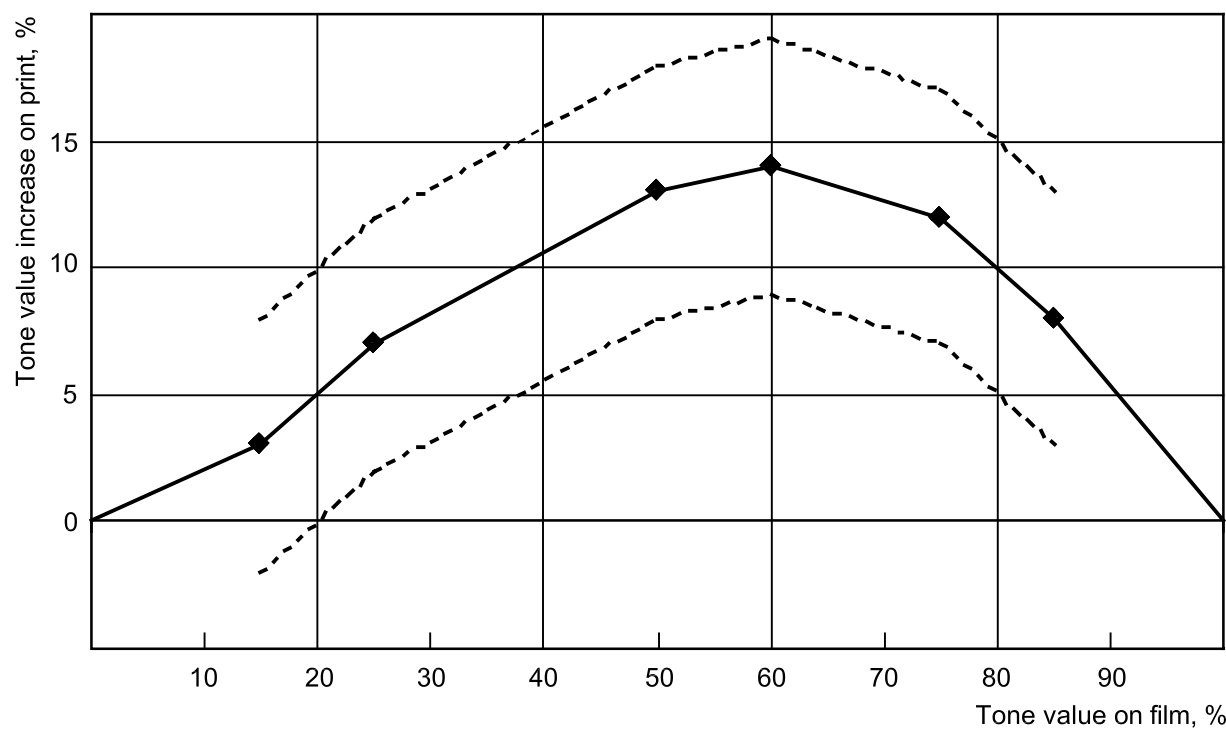
Figure 4 — Typical tone value increase curves for conventional UV and water-based air-dried ink (solid) and tolerances (broken), as measured at 30 cm -1
