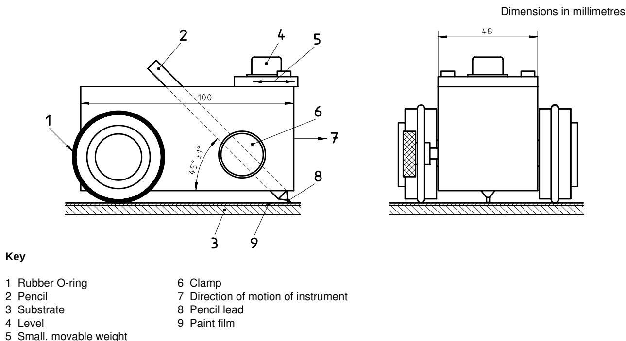
Figure 1 — Schematic diagram of test instrument
