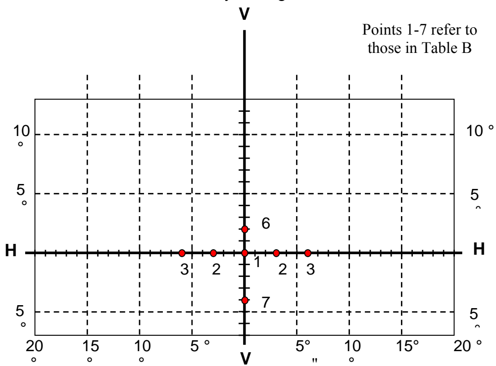
Figure E Secondary Driving Beam
