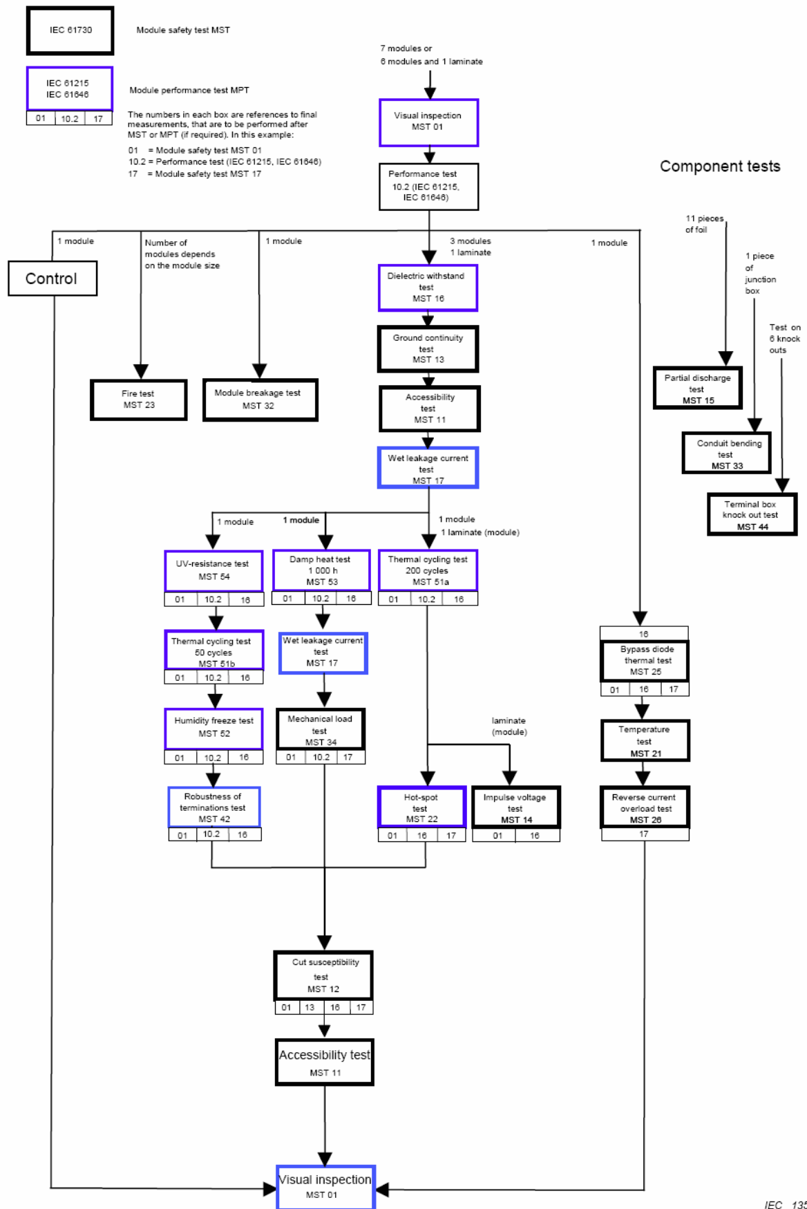
Figure 1 – Test sequences
